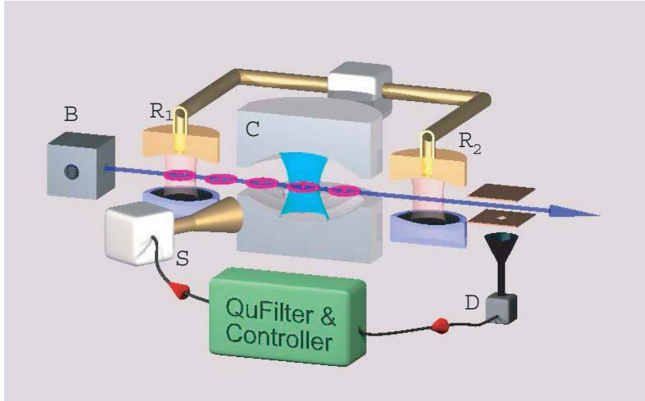
Figure 3.2: A schematic of the closed-loop system borrowed from [30]: an appropriate coherent pulse with a controlled amplitude and phase is injected between two atom passages.
