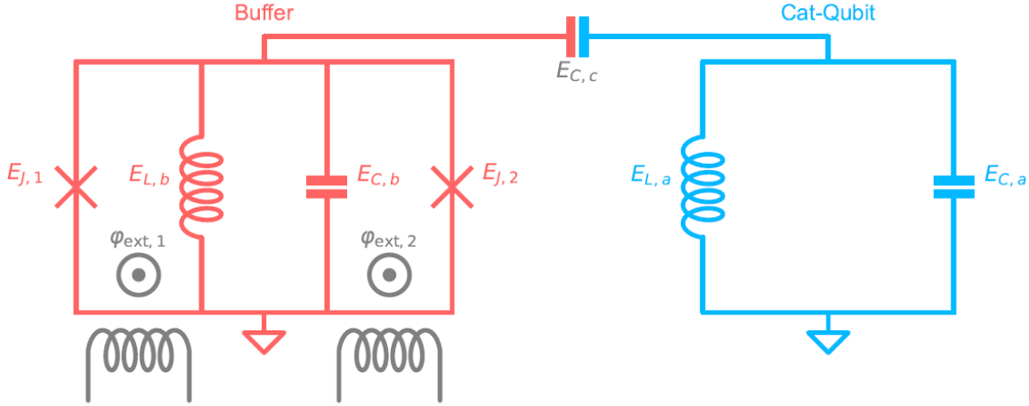
Figure 4.1: The super-conducting quantum circuit of [43, figure S3] stabilizes Schrödinger phase-cats of the high-quality oscillator \mathbf{a} with pulsation \omega_a (in blue) via nonlinear (Josephson junctions) and oscillatory (pulsation 2\omega_a - \omega_b ) Hamiltonian coupling to a low quality oscillator \mathbf{b} of pulsation \omega_b (in red).
