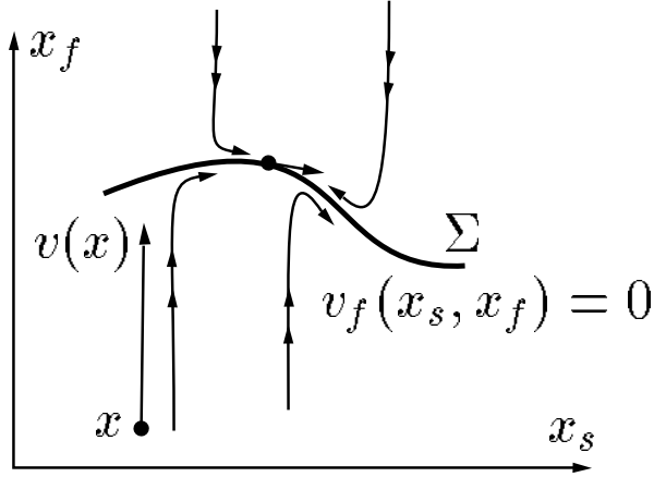
Figure G.2: Tikhonov normal form when the vector-field v = (v_s, v_f) is quasi vertical in the x = (x_s, x_f) coordinates.
