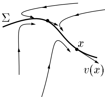
Figure G.1: Model reduction seen as restriction of the dynamics to an invariant attractive sub-manifold of the state manifold
