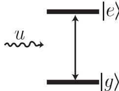
Figure 1.1: a 2-level system
