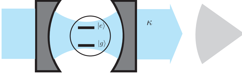
Figure 4.2: The cavity field interacts with the qubit and the cavity output gets measured providing information on the state of the qubit.
