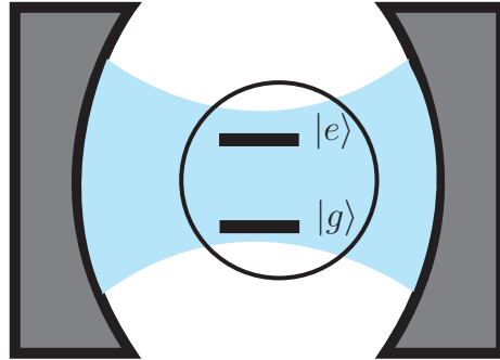
Figure 1.2: A composite spin-spring system: two-level atom coupled to quantized electromagnetic field confined in a cavity mode.
