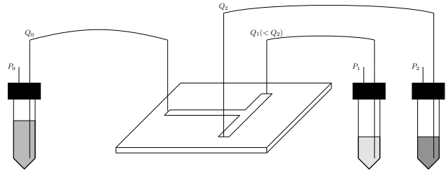
Fig. 1. Example of a microfluidic process [19]. Particles in a fluid are separated in the bifurcation point at a volume ratio that depends on flow rates Q_1, Q_2 of each daughter branch, which in turn can be manipulated via the respective pressures P_1, P_2 in the reservoirs.
